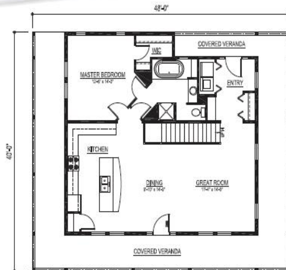
Main Plan
