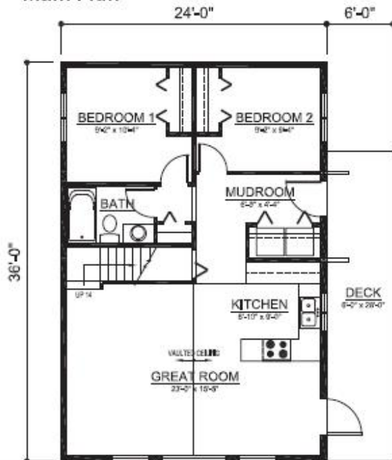
Main Plan
